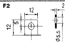
F2: Bold Fastened Terminal
