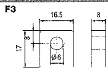
F3: Bold Fastened Terminal
