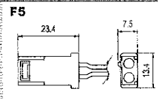
F5: Wire and connector
